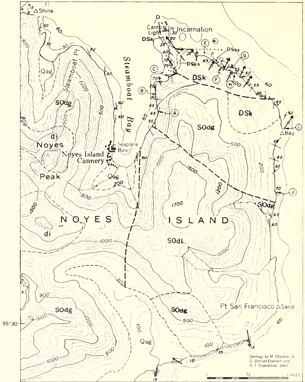
GEOLOGIC MAP OF NORTHEASTERN NOYES ISLAND, SOUTHEASTERN ALASKA
